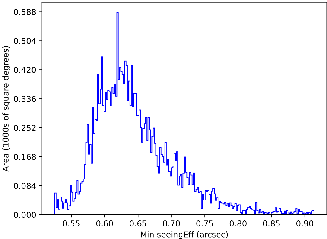
too_elab_r16_d3_griz_v3.4_10yrs All sky y band: Min seeingEff
