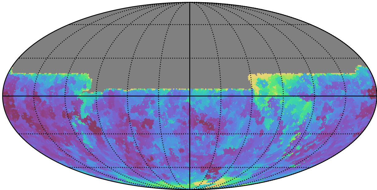
too_elab_r16_d3_griz_v3.4_10yrs All sky u band: Min seeingEff
