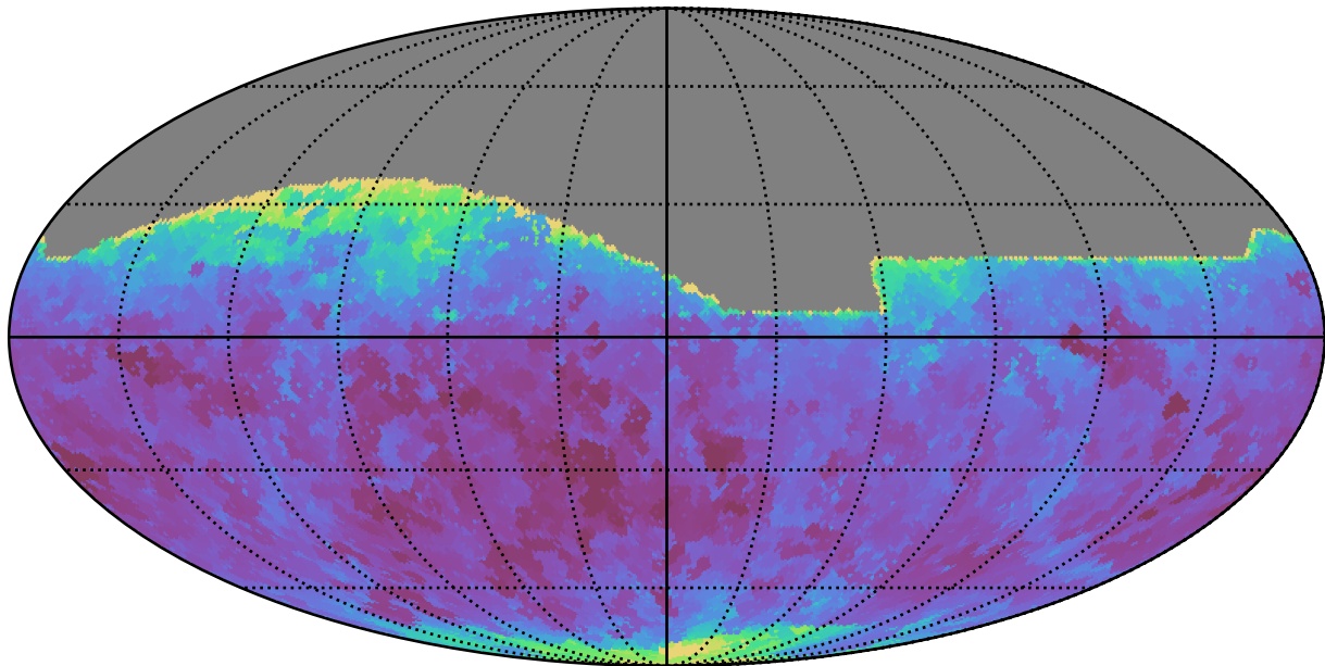
too_elab_r16_d3_griz_v3.4_10yrs All sky i band: Min seeingEff
