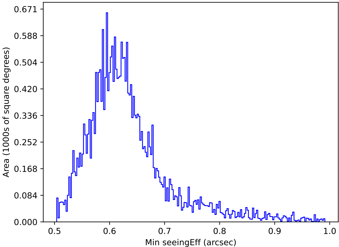
too_elab_r16_d3_griz_v3.4_10yrs All sky i band: Min seeingEff
