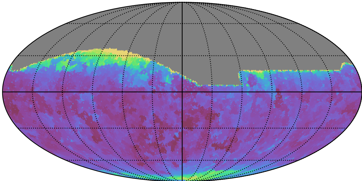
too_elab_r16_d3_griz_v3.4_10yrs All sky g band: Min seeingEff
