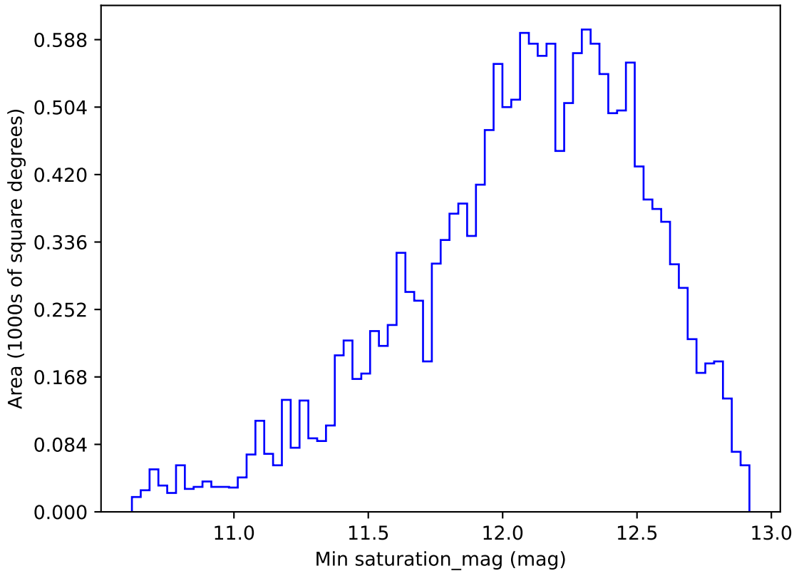
too_elab_r16_d3_griz_v3.4_10yrs WFD z band: Min saturation_mag
