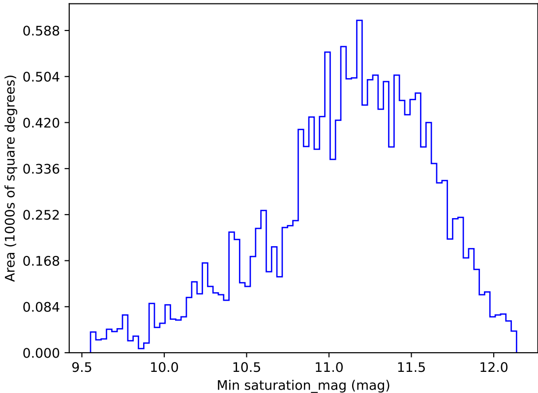
too_elab_r16_d3_griz_v3.4_10yrs WFD y band: Min saturation_mag
