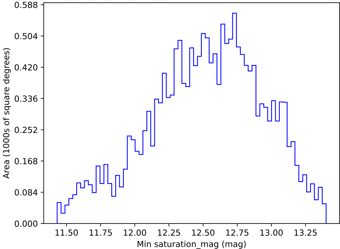
too_elab_r16_d3_griz_v3.4_10yrs WFD r band: Min saturation_mag
