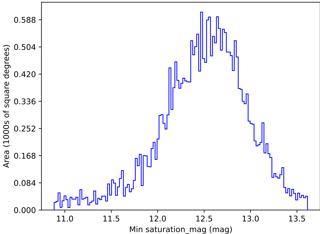
too_elab_r16_d3_griz_v3.4_10yrs All sky i band: Min saturation_mag
