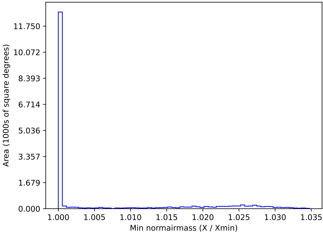
too_elab_r16_d3_griz_v3.4_10yrs WFD z band: Min normairmass
