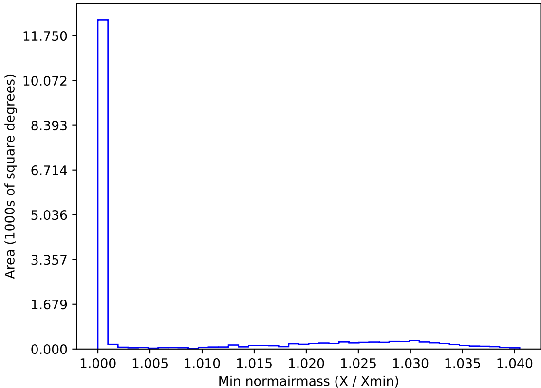
too_elab_r16_d3_griz_v3.4_10yrs WFD y band: Min normairmass
