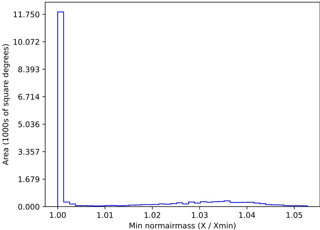
too_elab_r16_d3_griz_v3.4_10yrs WFD u band: Min normairmass
