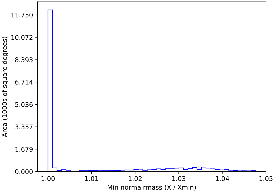
too_elab_r16_d3_griz_v3.4_10yrs WFD g band: Min normairmass
