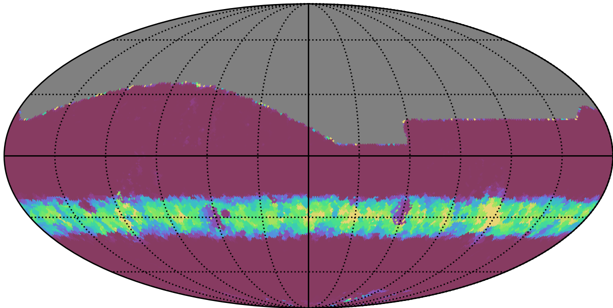
too_elab_r16_d3_griz_v3.4_10yrs All sky r band: Min normairmass
