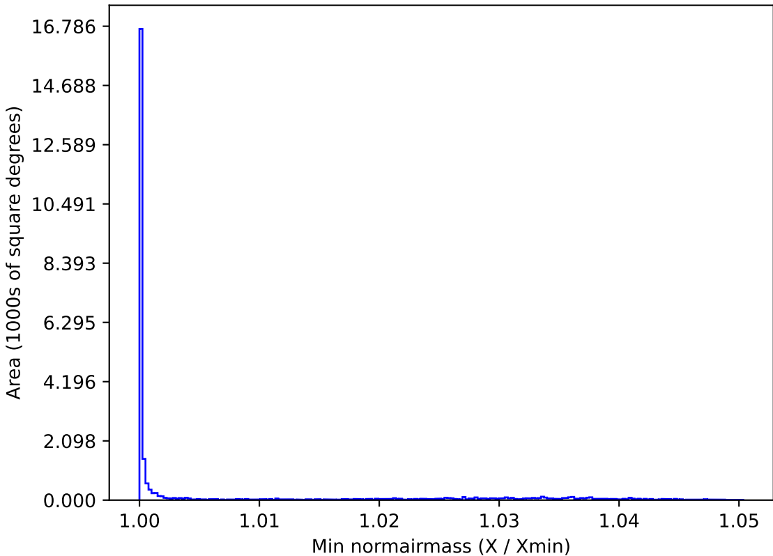
too_elab_r16_d3_griz_v3.4_10yrs All sky g band: Min normairmass
