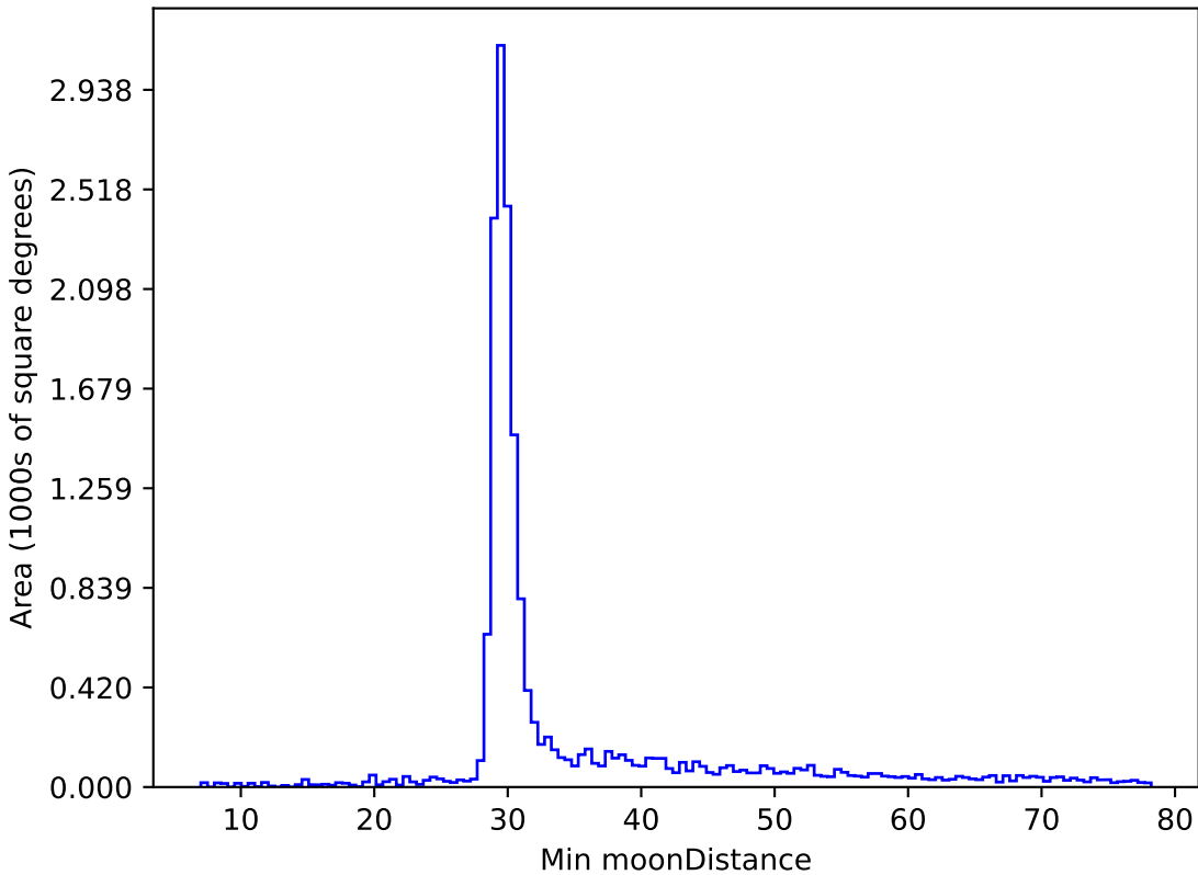
too_elab_r16_d3_griz_v3.4_10yrs WFD z band: Min moonDistance
