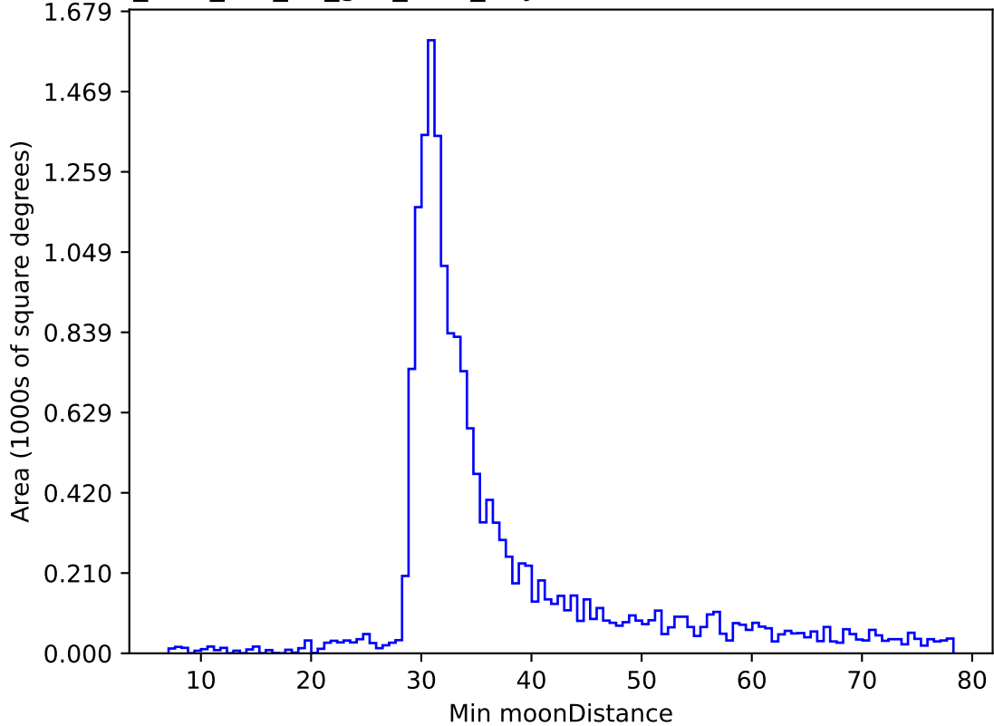
too_elab_r16_d3_griz_v3.4_10yrs WFD r band: Min moonDistance
