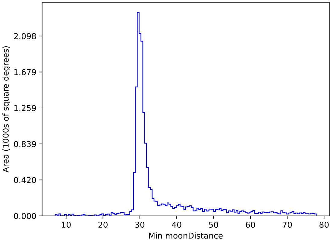
too_elab_r16_d3_griz_v3.4_10yrs WFD i band: Min moonDistance
