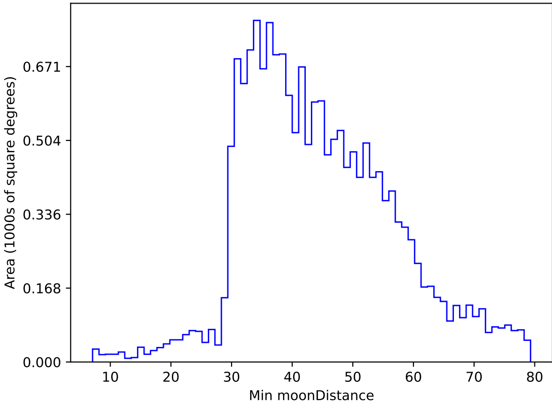
too_elab_r16_d3_griz_v3.4_10yrs WFD g band: Min moonDistance
