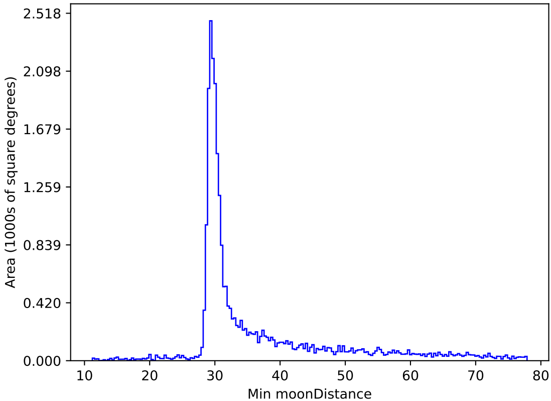
too_elab_r16_d3_griz_v3.4_10yrs All sky z band: Min moonDistance
