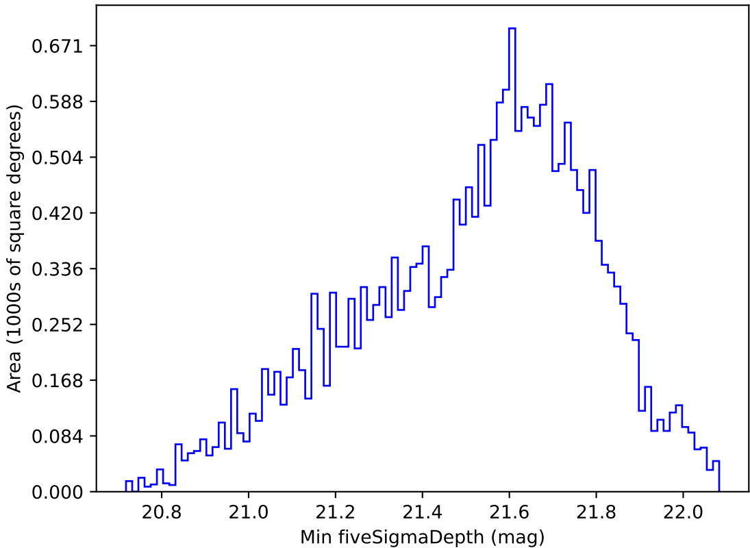
too_elab_r16_d3_griz_v3.4_10yrs Yr 1 y band: Min fiveSigmaDepth
