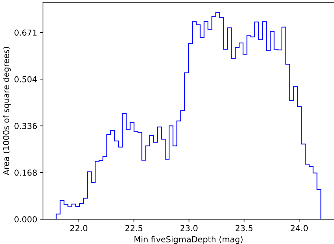
too_elab_r16_d3_griz_v3.4_10yrs Yr 1 r band: Min fiveSigmaDepth
