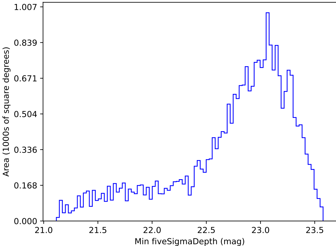
too_elab_r16_d3_griz_v3.4_10yrs Yr 1 i band: Min fiveSigmaDepth
