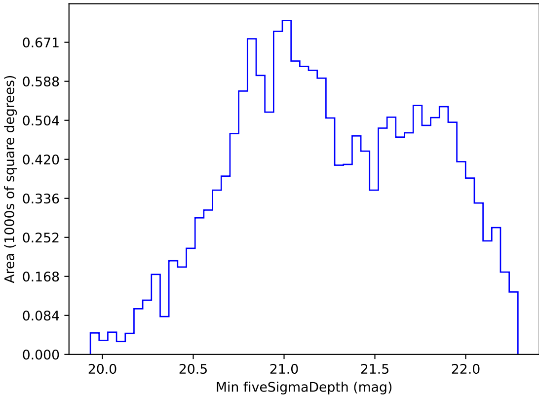
too_elab_r16_d3_griz_v3.4_10yrs WFD z band: Min fiveSigmaDepth
