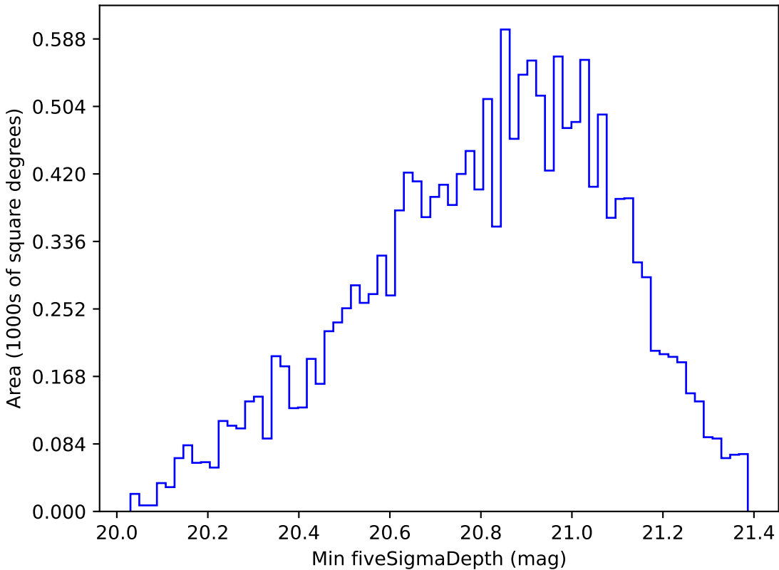
too_elab_r16_d3_griz_v3.4_10yrs WFD y band: Min fiveSigmaDepth
