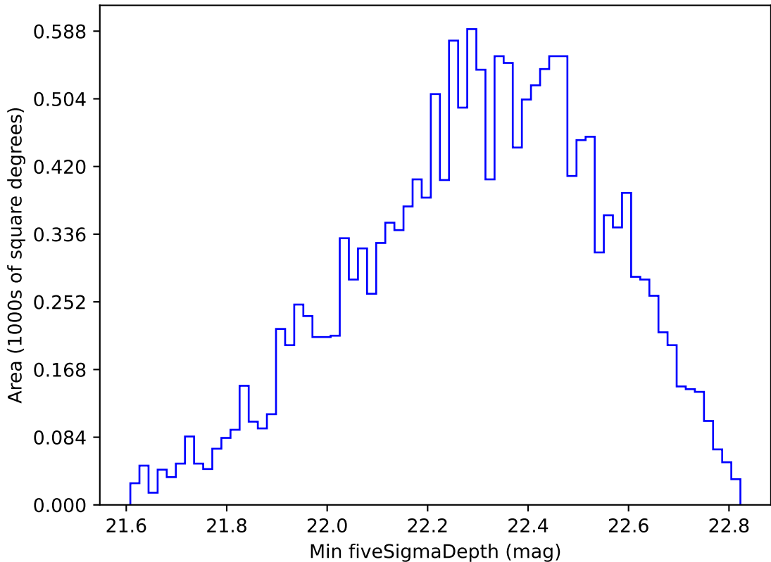
too_elab_r16_d3_griz_v3.4_10yrs WFD u band: Min fiveSigmaDepth
