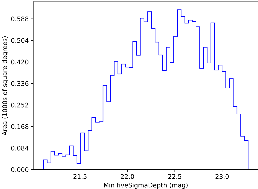
too_elab_r16_d3_griz_v3.4_10yrs WFD r band: Min fiveSigmaDepth
