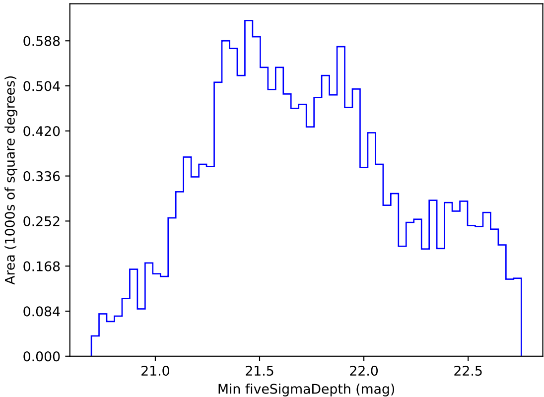
too_elab_r16_d3_griz_v3.4_10yrs WFD i band: Min fiveSigmaDepth
