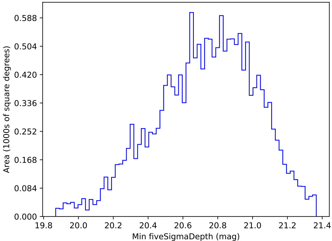
too_elab_r16_d3_griz_v3.4_10yrs WFD all bands: Min fiveSigmaDepth
