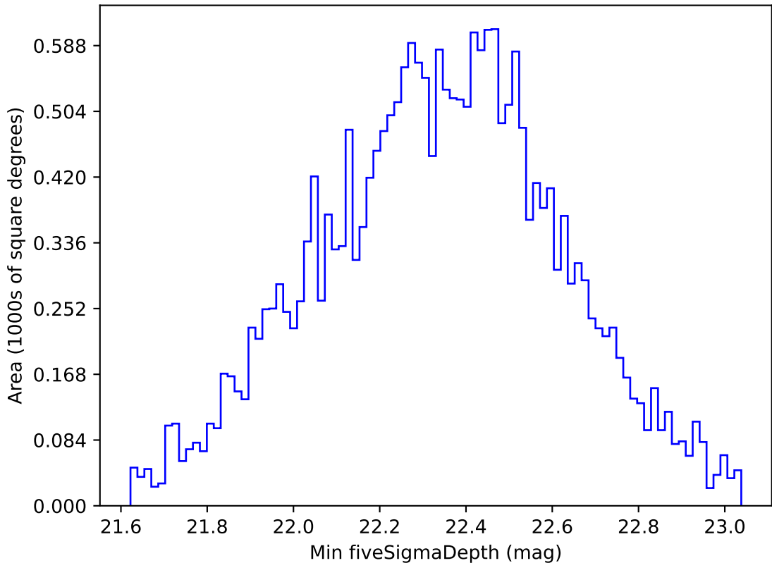
too_elab_r16_d3_griz_v3.4_10yrs All sky u band: Min fiveSigmaDepth
