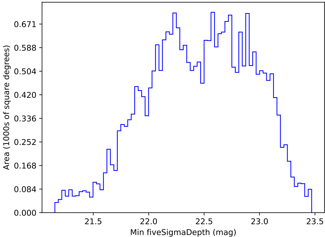
too_elab_r16_d3_griz_v3.4_10yrs All sky r band: Min fiveSigmaDepth
