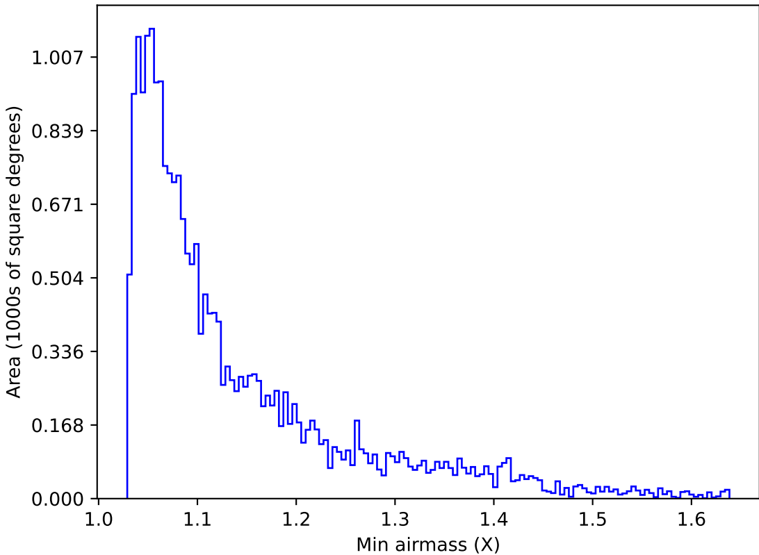
too_elab_r16_d3_griz_v3.4_10yrs Yr 1 u band: Min airmass
