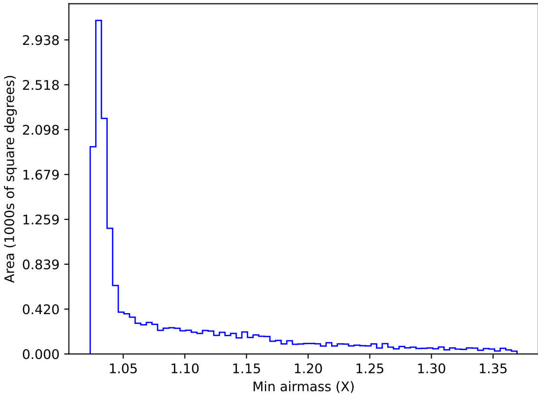
too_elab_r16_d3_griz_v3.4_10yrs WFD y band: Min airmass
