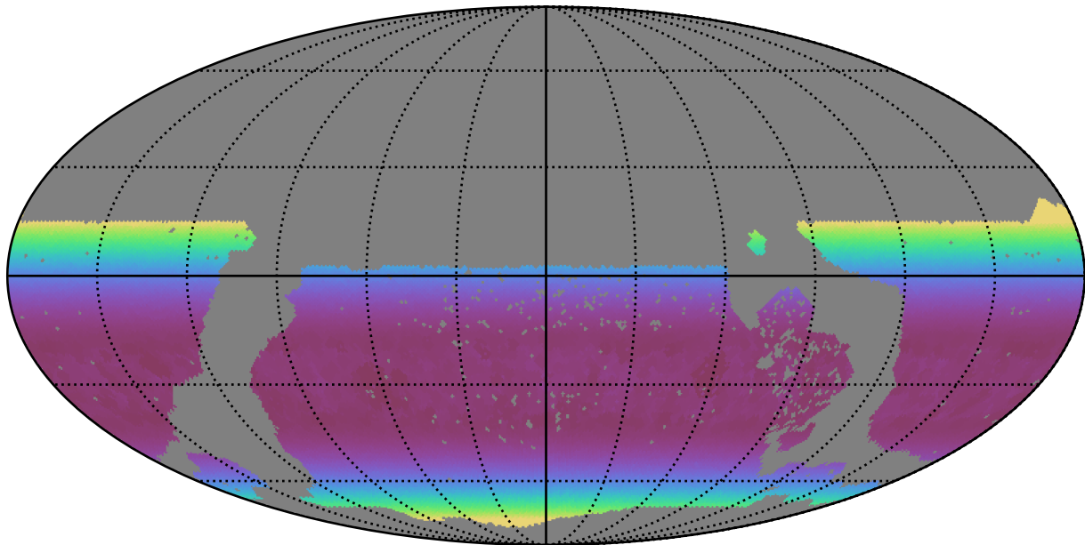
too_elab_r16_d3_griz_v3.4_10yrs WFD r band: Min airmass
