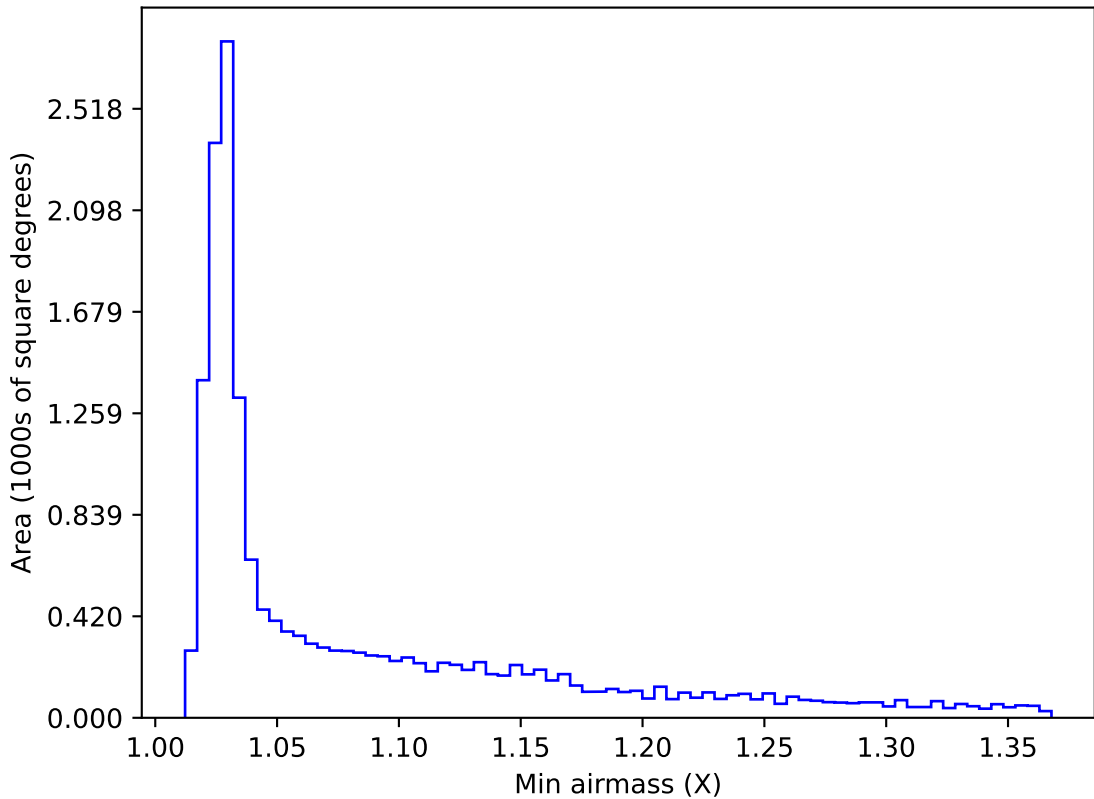
too_elab_r16_d3_griz_v3.4_10yrs WFD r band: Min airmass
