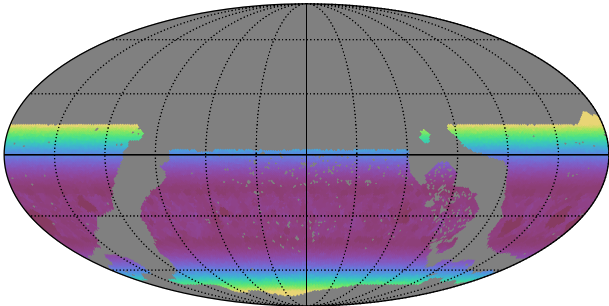
too_elab_r16_d3_griz_v3.4_10yrs WFD g band: Min airmass
