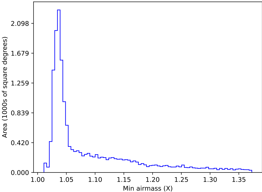
too_elab_r16_d3_griz_v3.4_10yrs WFD g band: Min airmass
