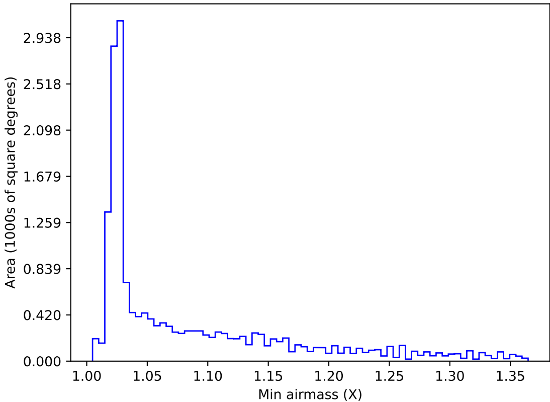
too_elab_r16_d3_griz_v3.4_10yrs WFD all bands: Min airmass
