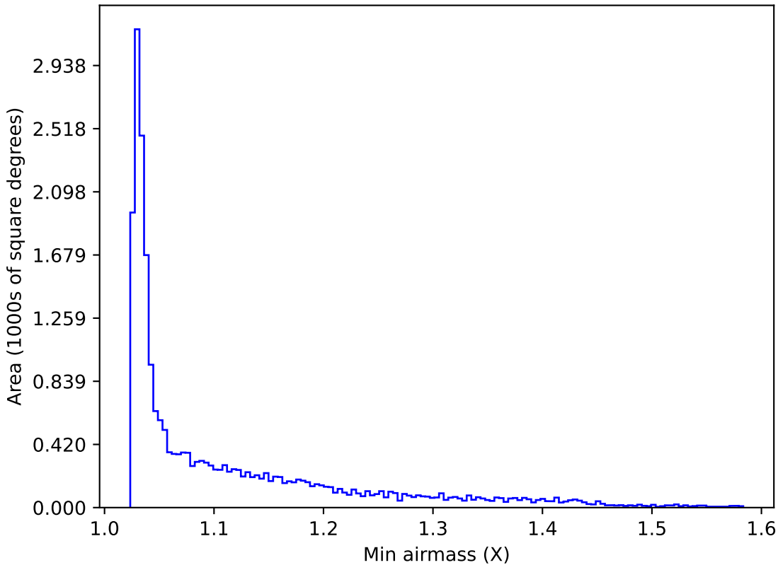
too_elab_r16_d3_griz_v3.4_10yrs All sky y band: Min airmass
