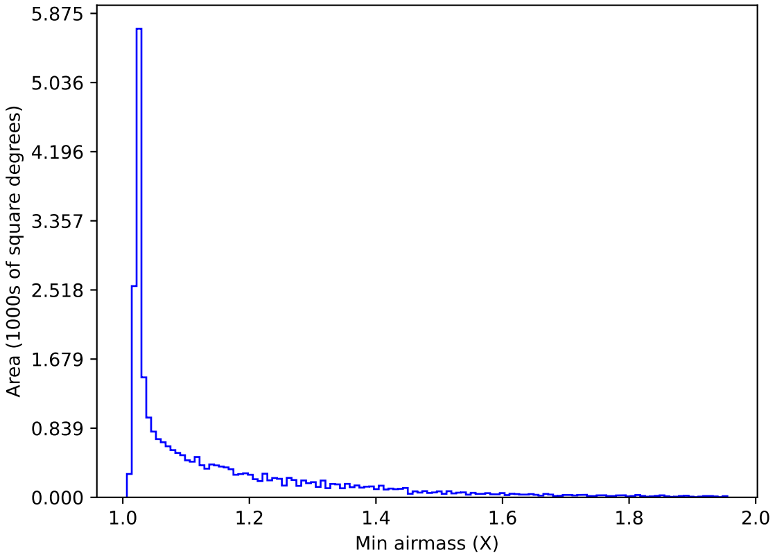
too_elab_r16_d3_griz_v3.4_10yrs All sky all bands: Min airmass
