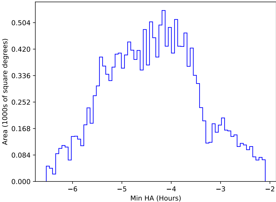
too_elab_r16_d3_griz_v3.4_10yrs WFD z band: Min HA
