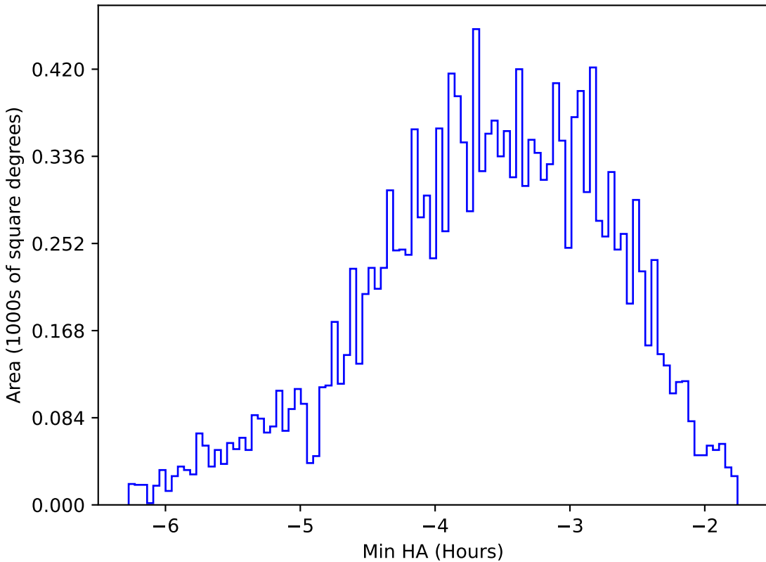
too_elab_r16_d3_griz_v3.4_10yrs WFD y band: Min HA
