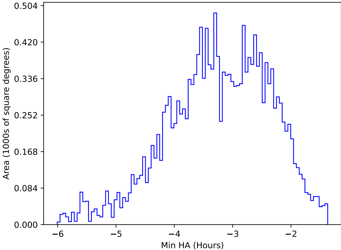
too_elab_r16_d3_griz_v3.4_10yrs WFD u band: Min HA
