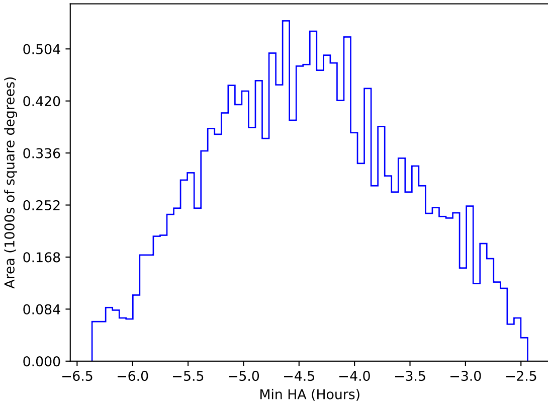
too_elab_r16_d3_griz_v3.4_10yrs WFD r band: Min HA
