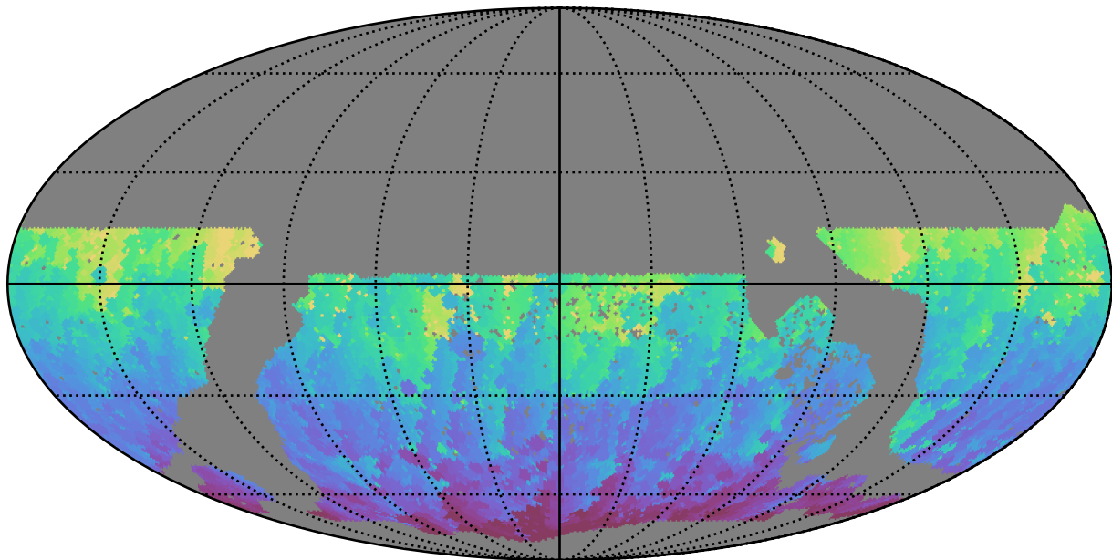
too_elab_r16_d3_griz_v3.4_10yrs WFD g band: Min HA
