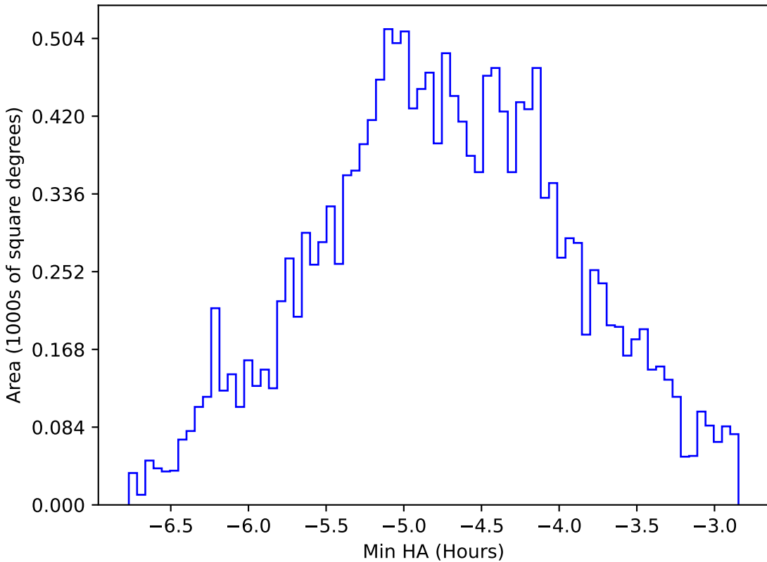
too_elab_r16_d3_griz_v3.4_10yrs WFD all bands: Min HA
