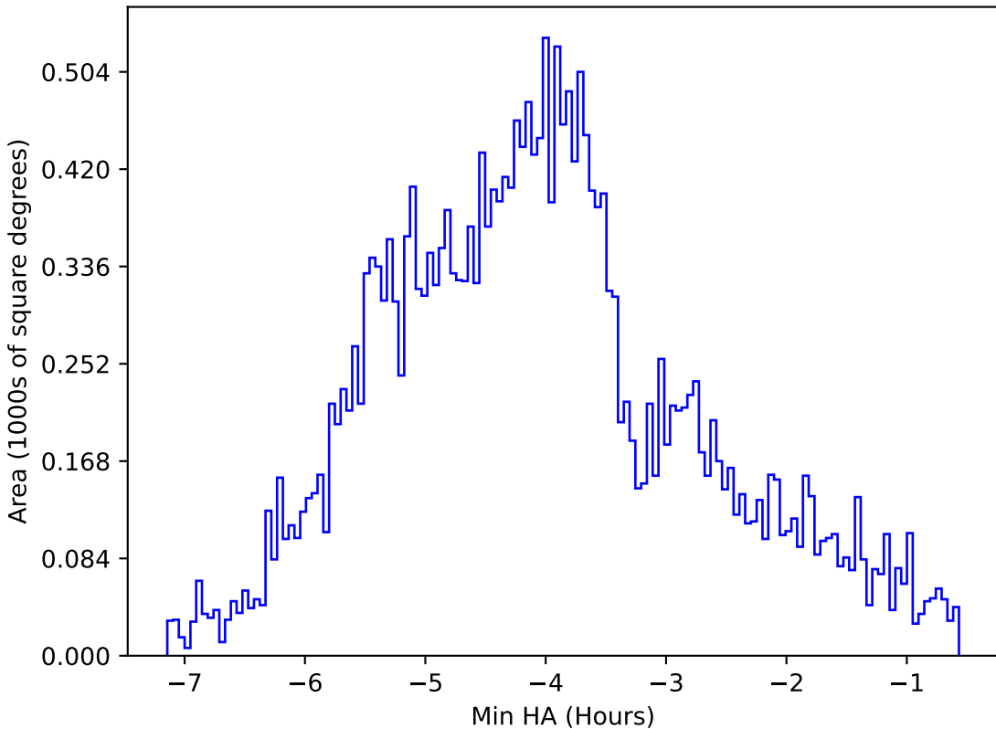
too_elab_r16_d3_griz_v3.4_10yrs All sky z band: Min HA
