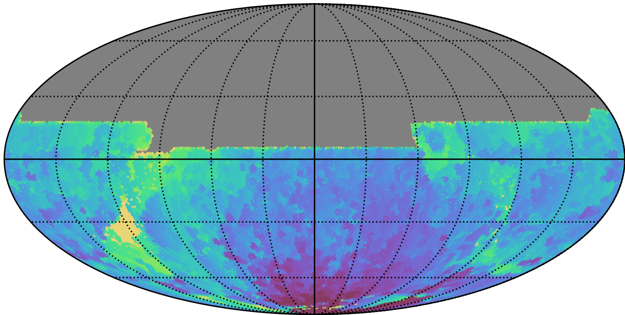
too_elab_r16_d3_griz_v3.4_10yrs All sky y band: Min HA
