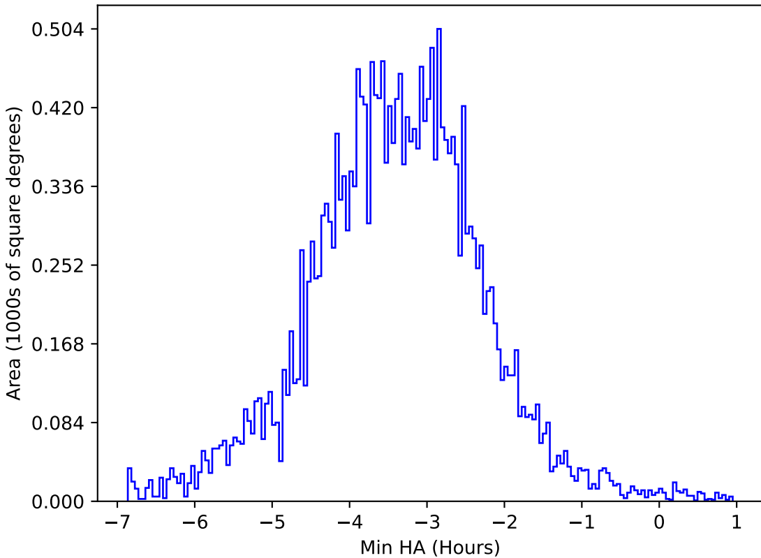
too_elab_r16_d3_griz_v3.4_10yrs All sky y band: Min HA
