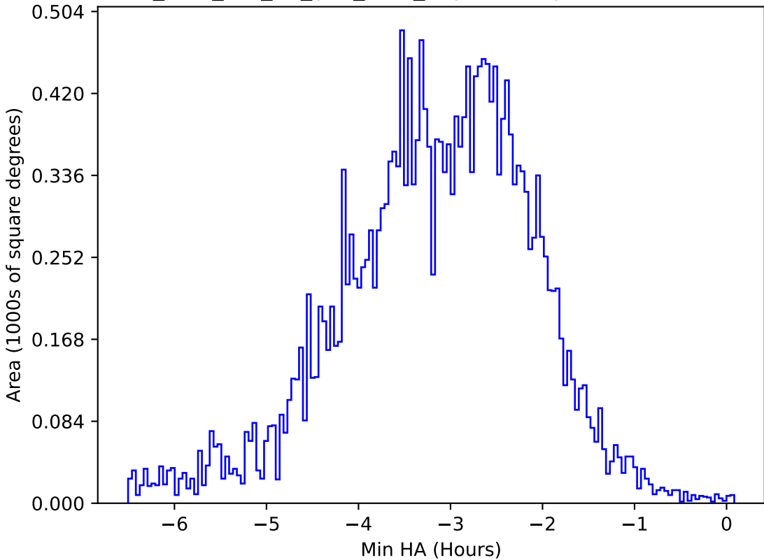
too_elab_r16_d3_griz_v3.4_10yrs All sky u band: Min HA
